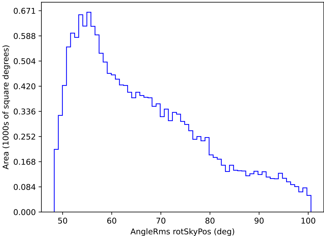
weather_cloudso30v3.4_10yrs WFD z band: AngleRms rotSkyPos
