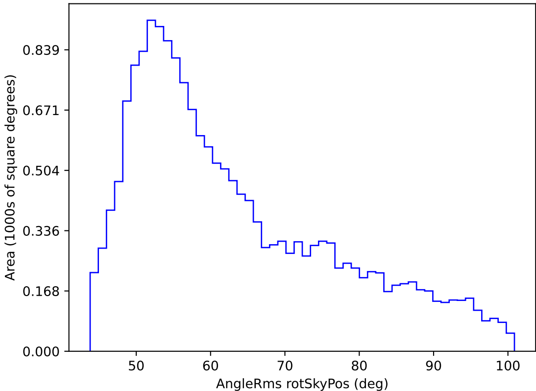
weather_cloudso30v3.4_10yrs WFD y band: AngleRms rotSkyPos
