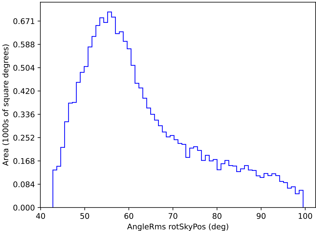
weather_cloudso30v3.4_10yrs WFD u band: AngleRms rotSkyPos
