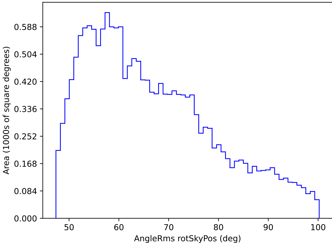
weather_cloudso30v3.4_10yrs WFD r band: AngleRms rotSkyPos
