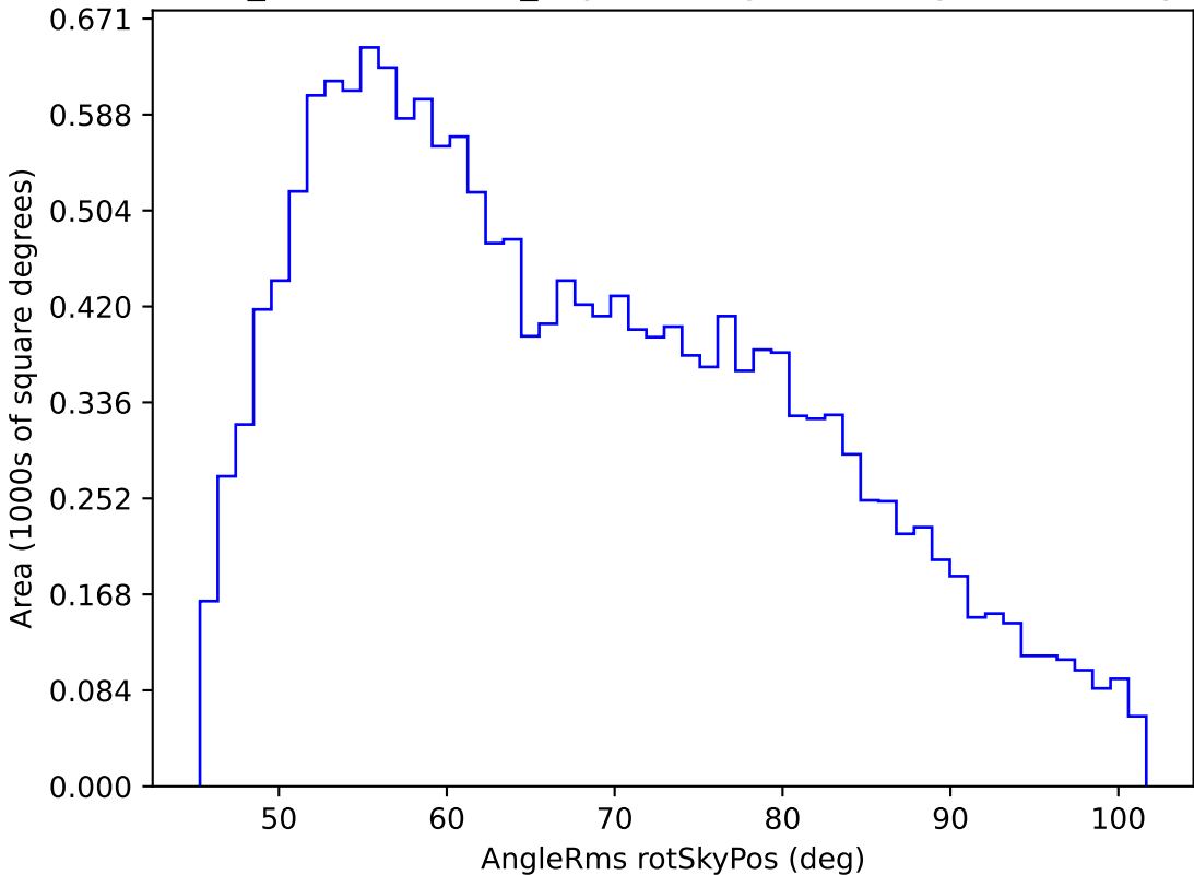
weather_cloudso30v3.4_10yrs WFD g band: AngleRms rotSkyPos
