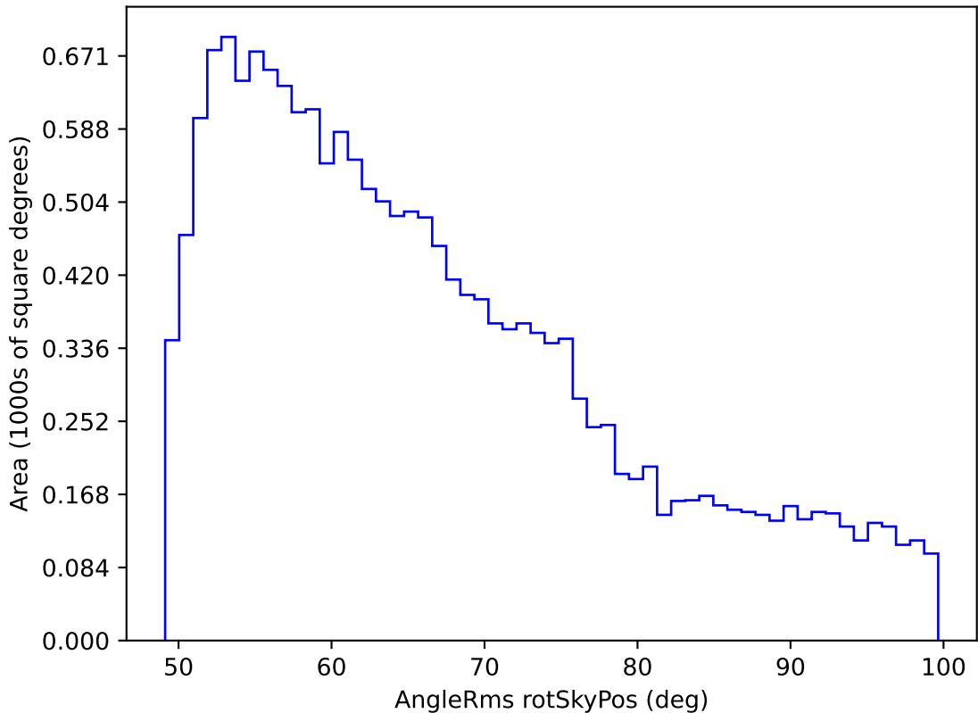
weather_cloudso30v3.4_10yrs WFD all bands: AngleRms rotSkyPos
