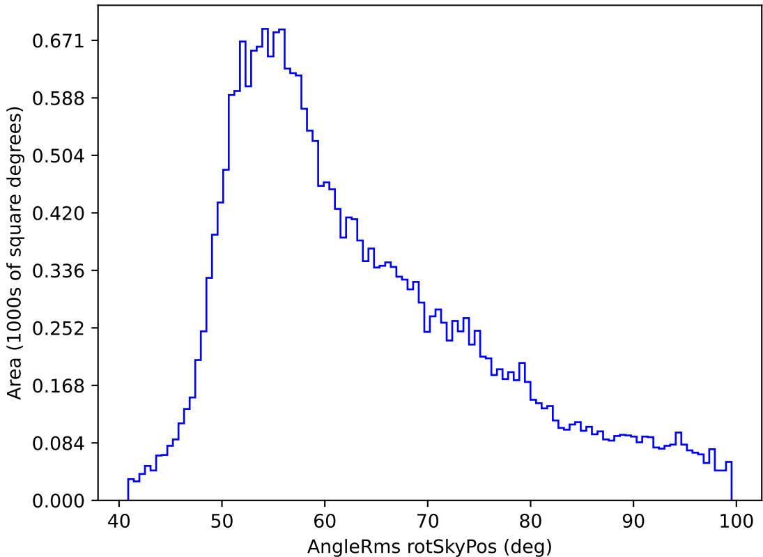
weather_cloudso30v3.4_10yrs All sky z band: AngleRms rotSkyPos
