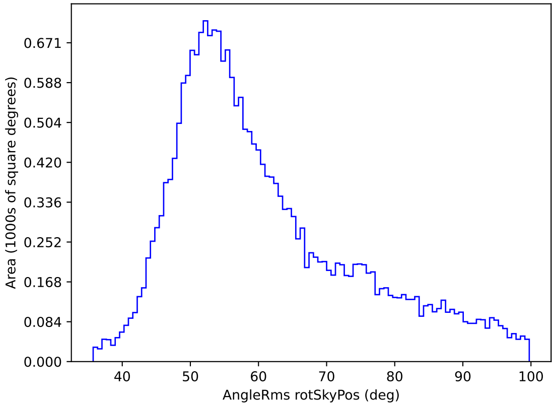
weather_cloudso30v3.4_10yrs All sky y band: AngleRms rotSkyPos
