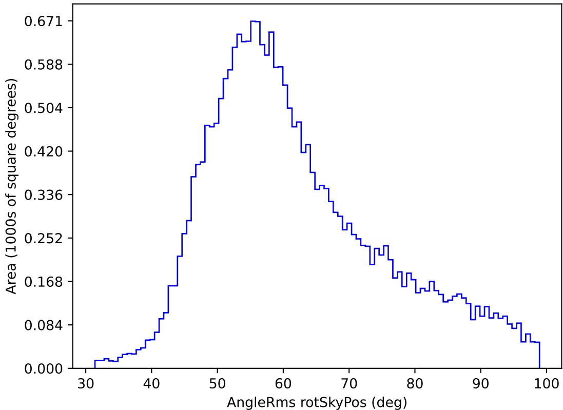
weather_cloudso30v3.4_10yrs All sky u band: AngleRms rotSkyPos
