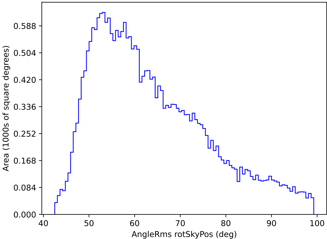
weather_cloudso30v3.4_10yrs All sky r band: AngleRms rotSkyPos
