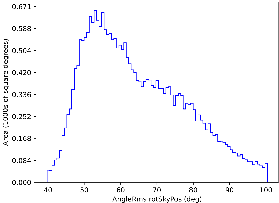
weather_cloudso30v3.4_10yrs All sky g band: AngleRms rotSkyPos
