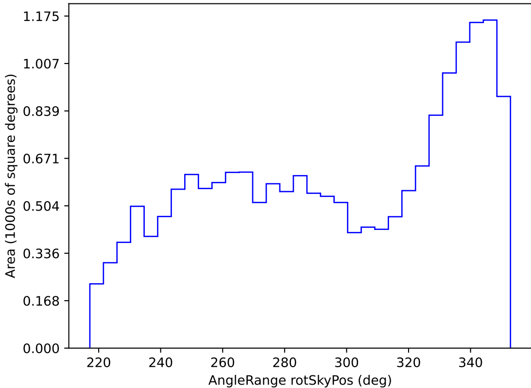
weather_cloudso30v3.4_10yrs WFD all bands: AngleRange rotSkyPos
