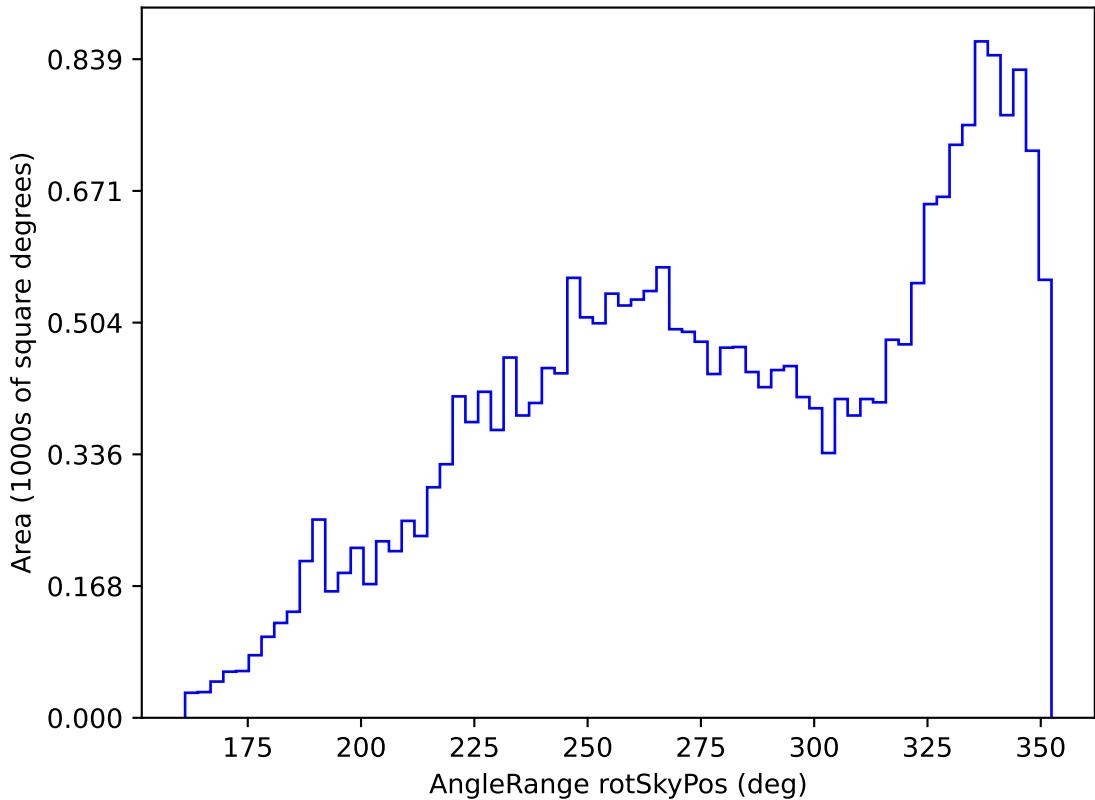
weather_cloudso30v3.4_10yrs All sky all bands: AngleRange rotSkyPos
