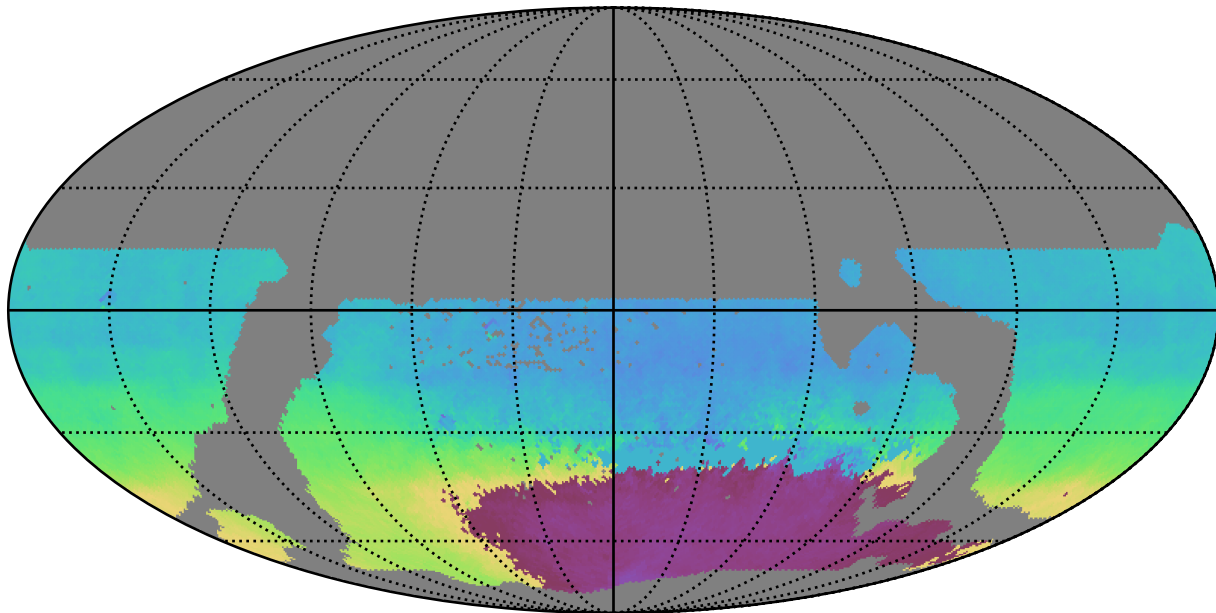
weather_cloudso30v3.4_10yrs WFD r band: AngleMean rotSkyPos
