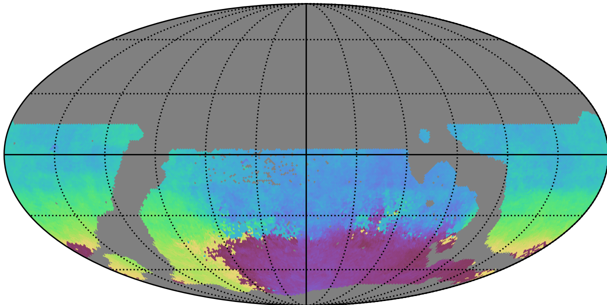
weather_cloudso30v3.4_10yrs WFD g band: AngleMean rotSkyPos
