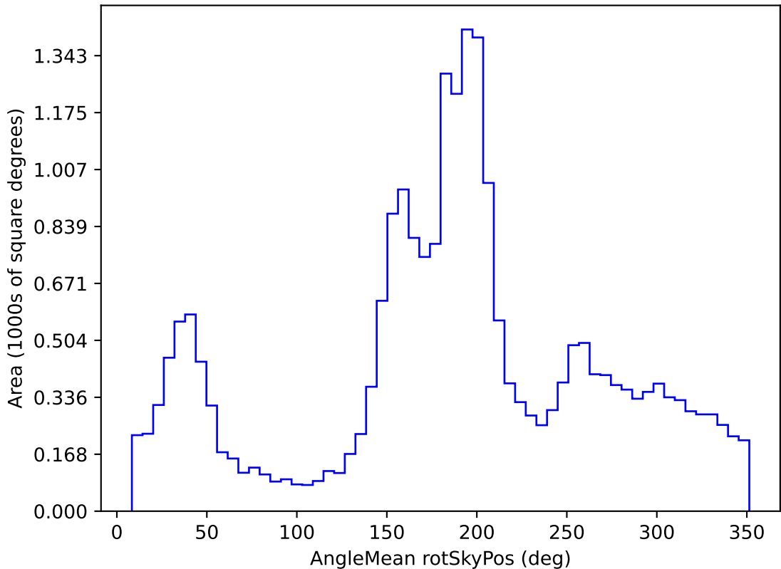
weather_cloudso30v3.4_10yrs All sky u band: AngleMean rotSkyPos
