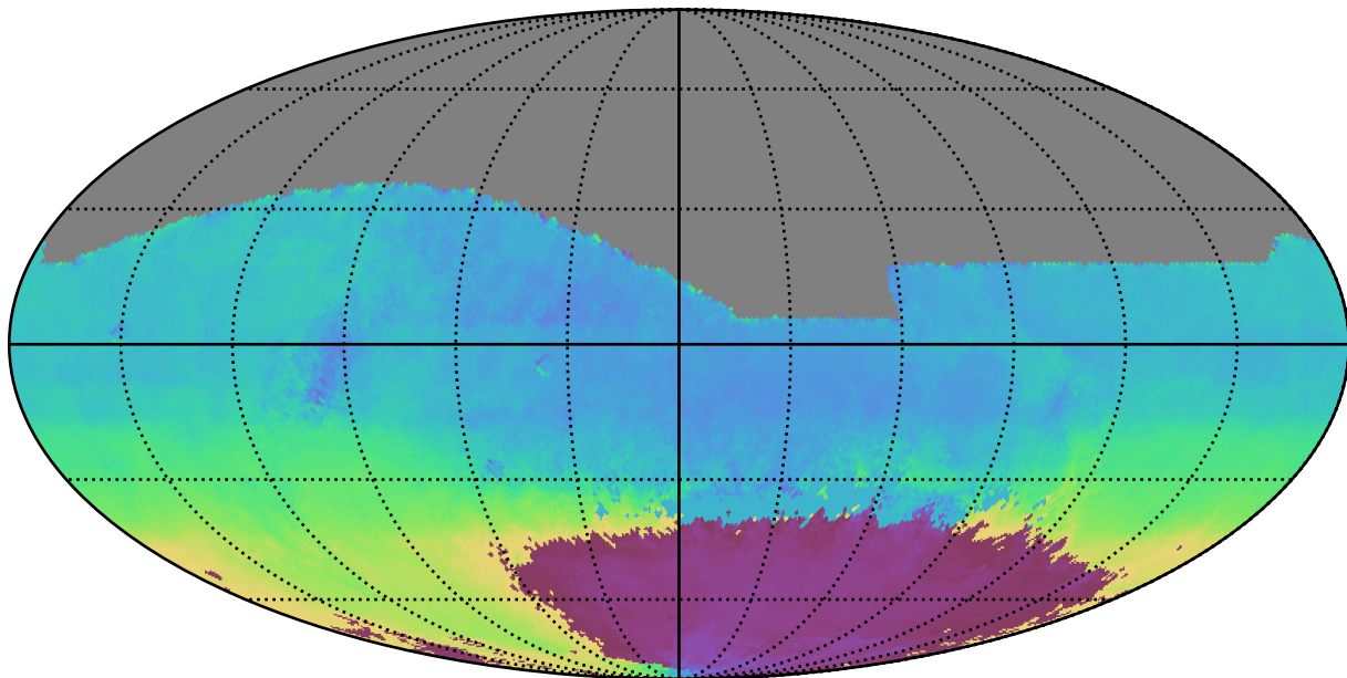
weather_cloudso30v3.4_10yrs All sky r band: AngleMean rotSkyPos
