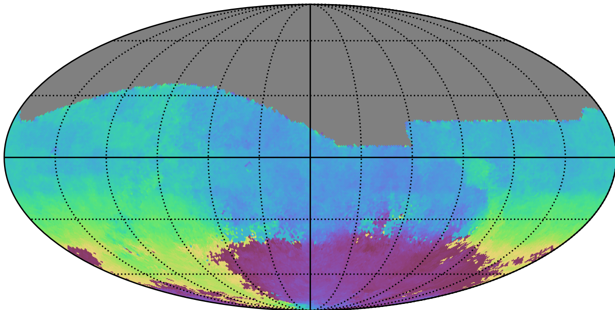
weather_cloudso30v3.4_10yrs All sky g band: AngleMean rotSkyPos
