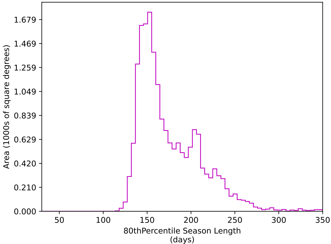
weather_cloudso30v3.4_10yrs WFD z band: 80thPercentile Season Length
