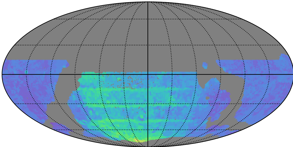
weather_cloudso30v3.4_10yrs WFD y band: 80thPercentile Season Length
