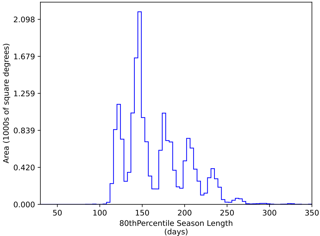
weather_cloudso30v3.4_10yrs WFD y band: 80thPercentile Season Length
