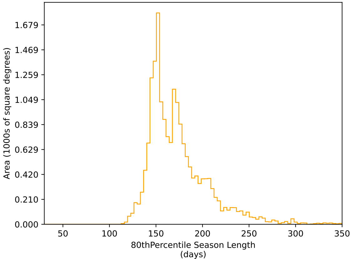
weather_cloudso30v3.4_10yrs WFD r band: 80thPercentile Season Length
