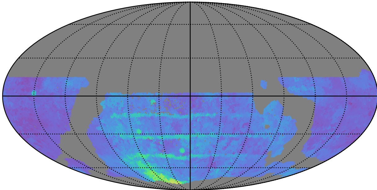
weather_cloudso30v3.4_10yrs WFD g band: 80thPercentile Season Length
