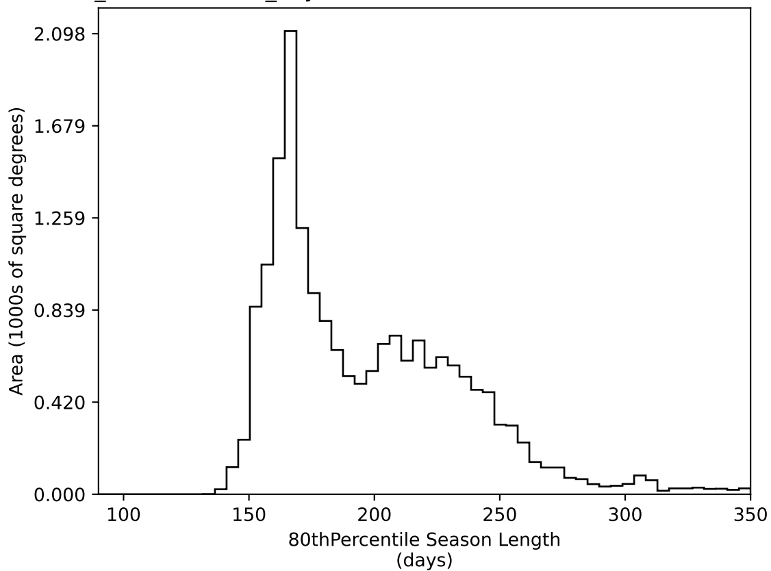
weather_cloudso30v3.4_10yrs WFD all bands: 80thPercentile Season Length
