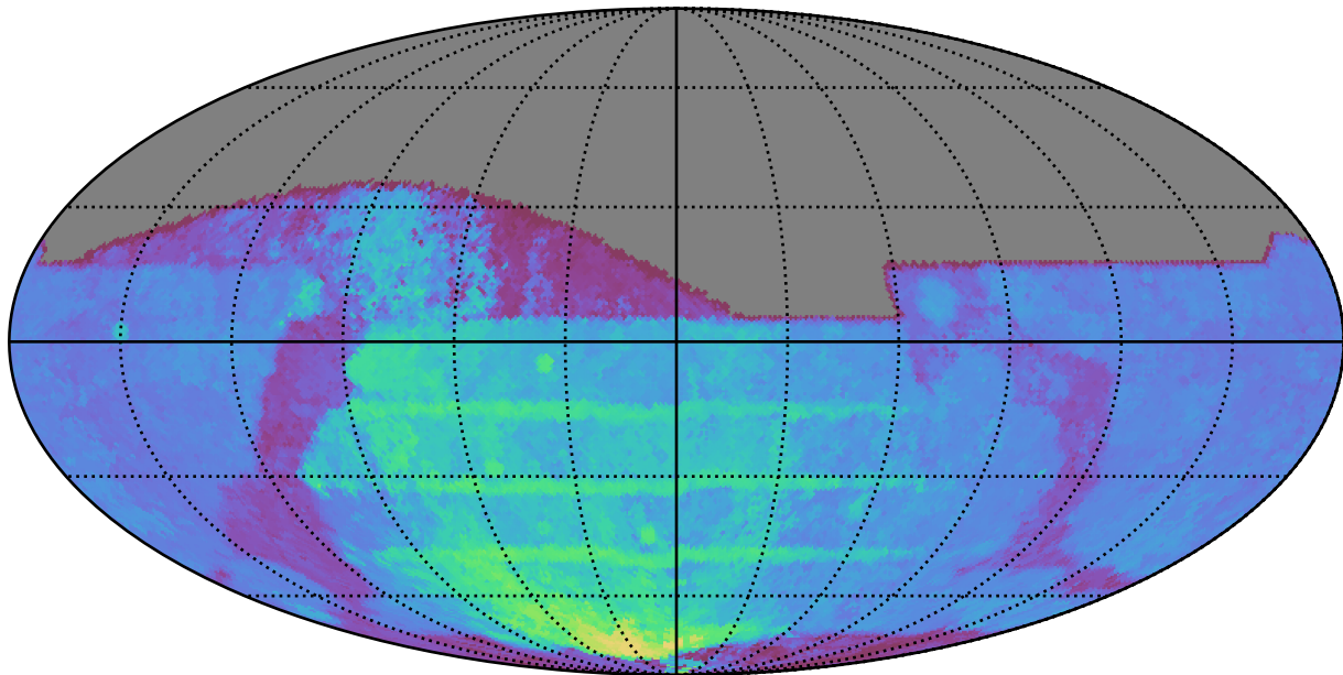
weather_cloudso30v3.4_10yrs All sky z band: 80thPercentile Season Length
