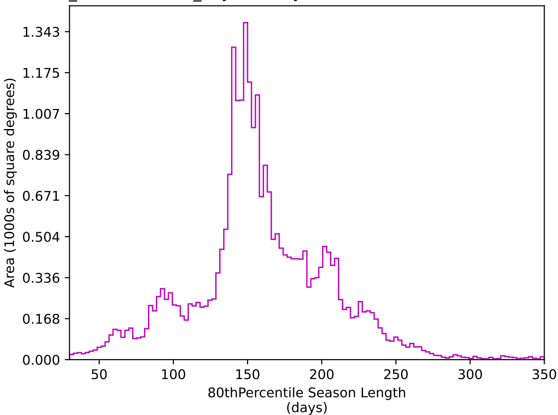
weather_cloudso30v3.4_10yrs All sky z band: 80thPercentile Season Length
