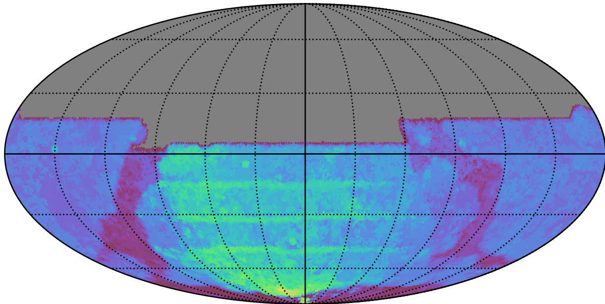
weather_cloudso30v3.4_10yrs All sky y band: 80thPercentile Season Length
