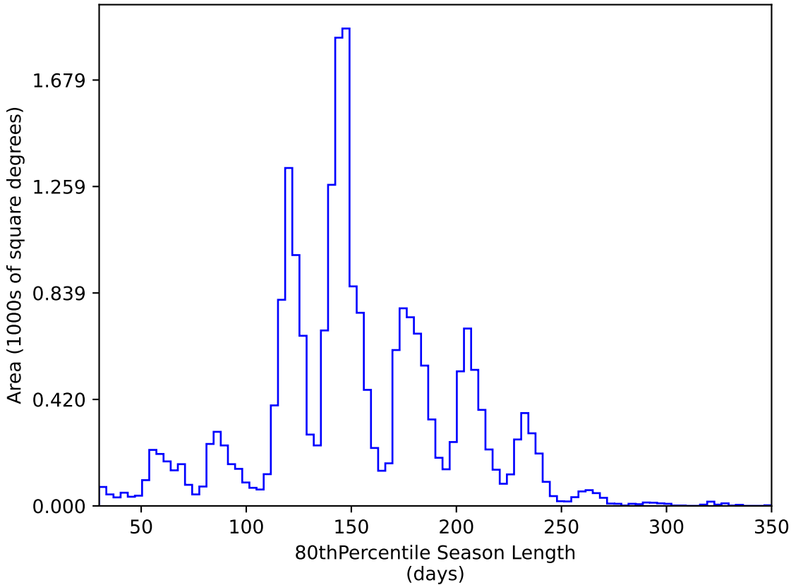
weather_cloudso30v3.4_10yrs All sky y band: 80thPercentile Season Length
