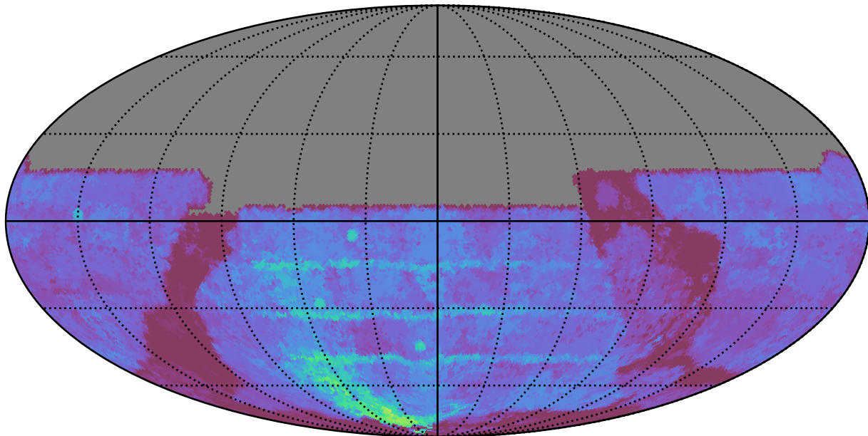
weather_cloudso30v3.4_10yrs All sky u band: 80thPercentile Season Length
