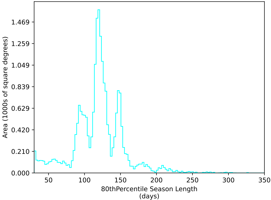
weather_cloudso30v3.4_10yrs All sky u band: 80thPercentile Season Length
