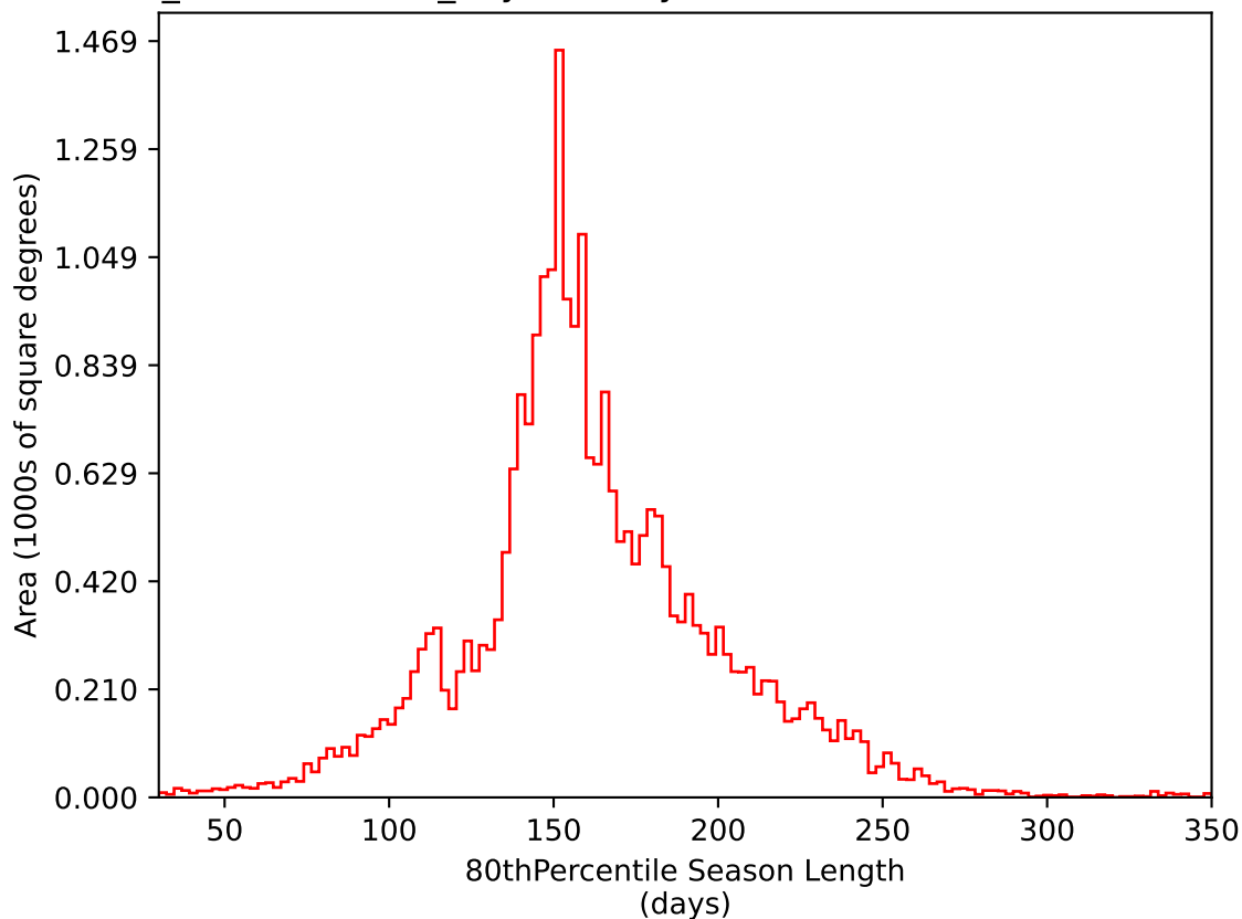
weather_cloudso30v3.4_10yrs All sky i band: 80thPercentile Season Length
