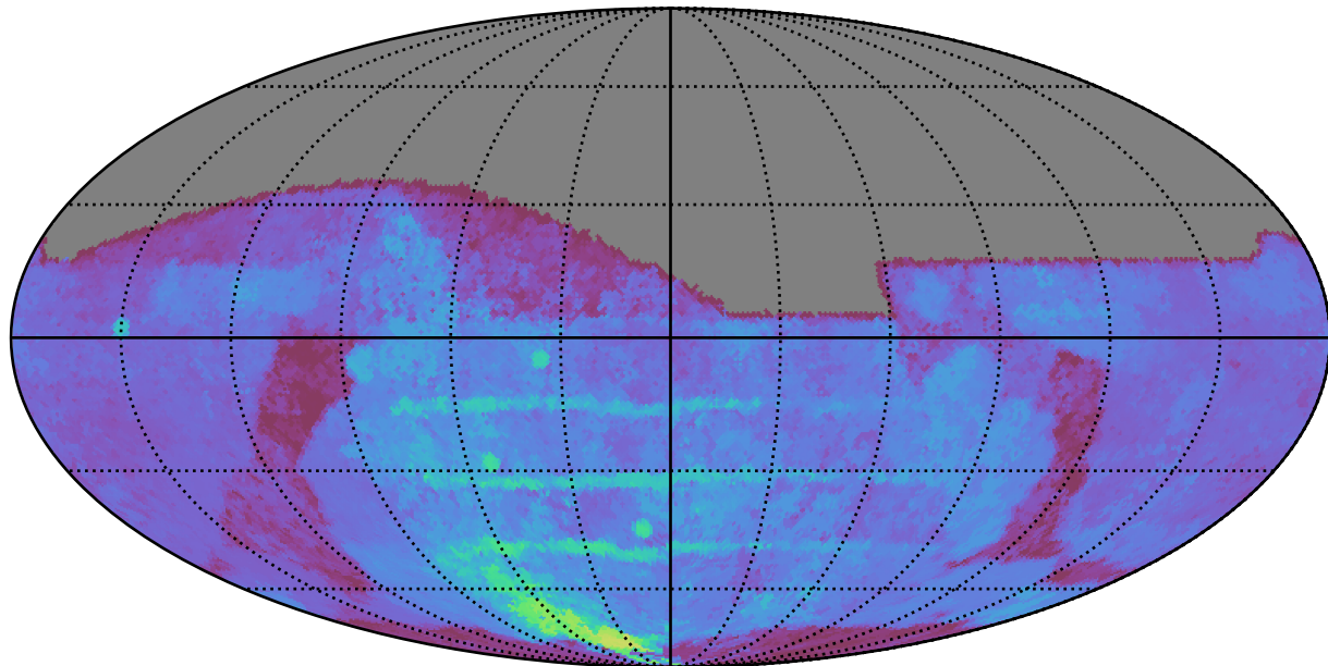
weather_cloudso30v3.4_10yrs All sky g band: 80thPercentile Season Length
