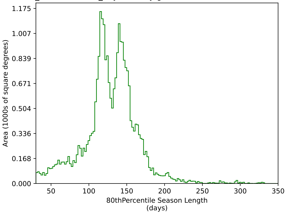
weather_cloudso30v3.4_10yrs All sky g band: 80thPercentile Season Length
