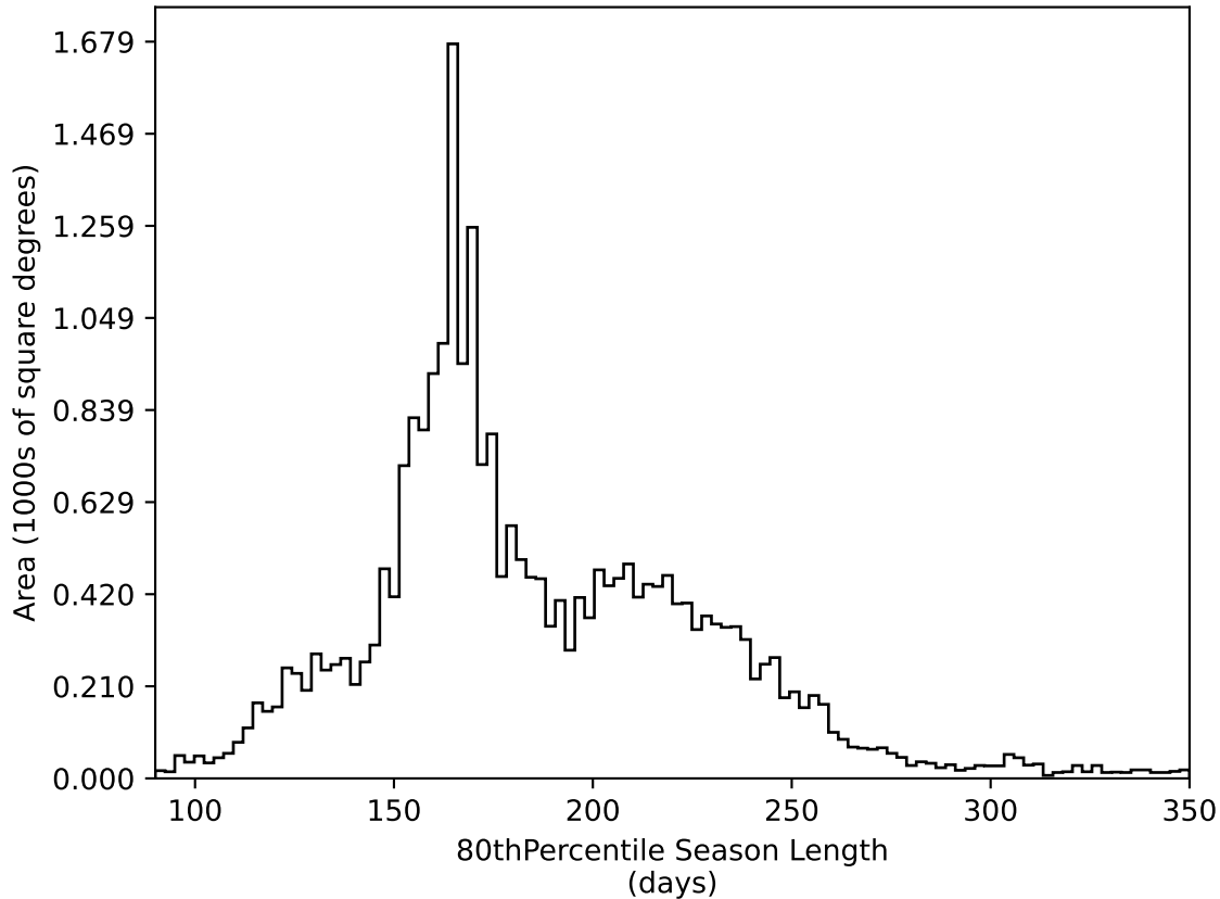
weather_cloudso30v3.4_10yrs All sky all bands: 80thPercentile Season Length
