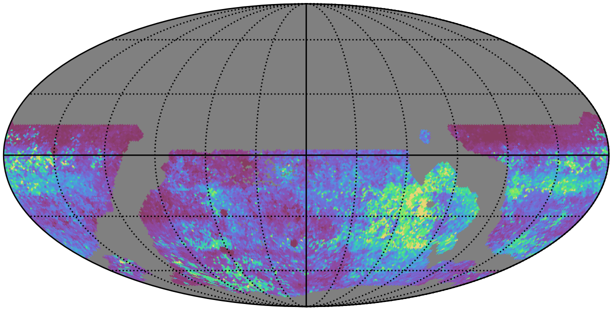
weather_cloudso30v3.4_10yrs WFD zy bands: 75th Percentile Intranight Timespan
