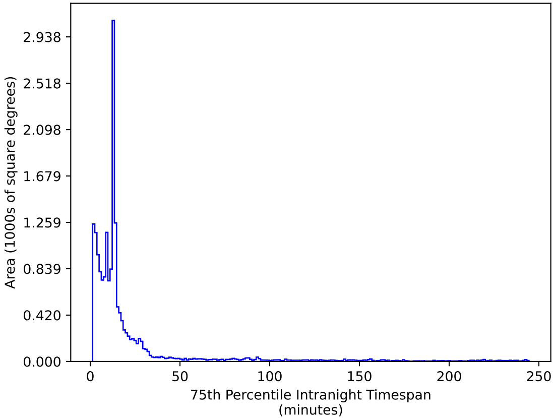
weather_cloudso30v3.4_10yrs WFD z band: 75th Percentile Intranight Timespan
