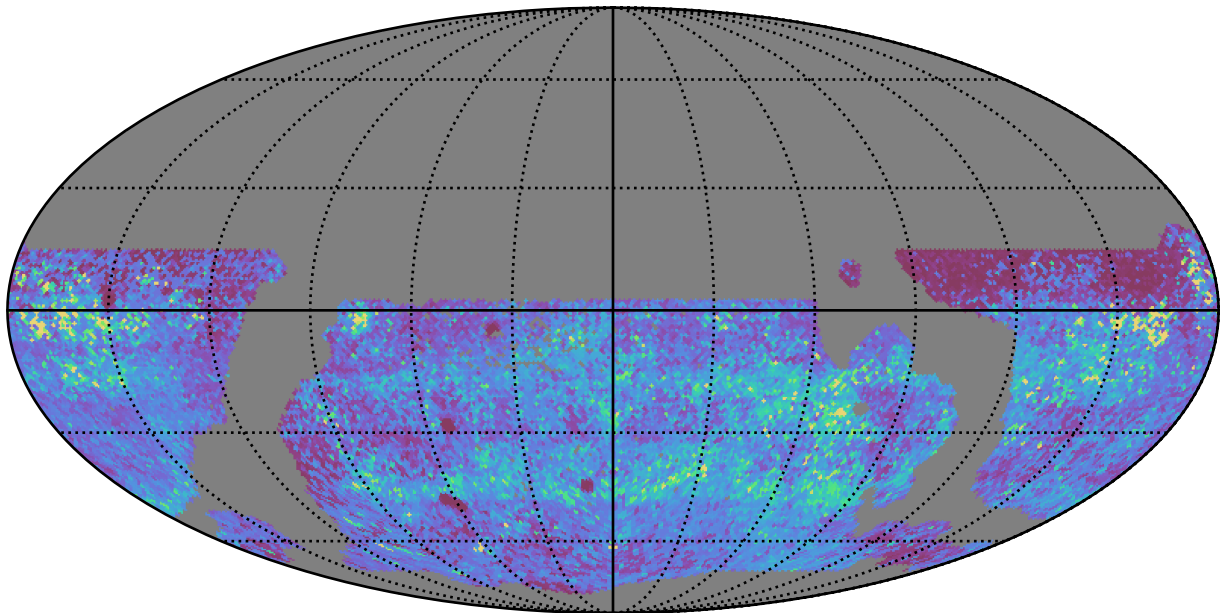
weather_cloudso30v3.4_10yrs WFD y band: 75th Percentile Intranight Timespan
