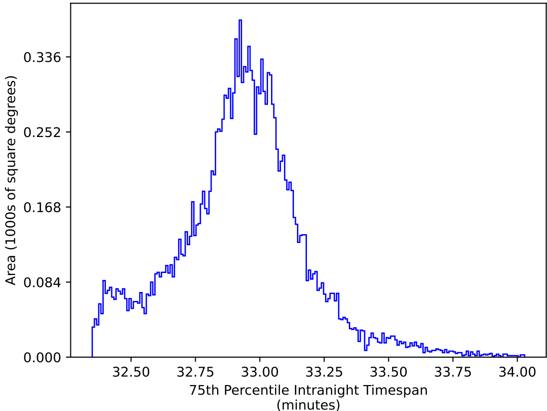
weather_cloudso30v3.4_10yrs WFD y band: 75th Percentile Intranight Timespan
