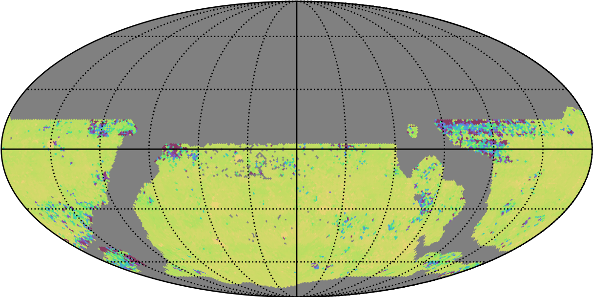
weather_cloudso30v3.4_10yrs WFD ug bands: 75th Percentile Intranight Timespan
