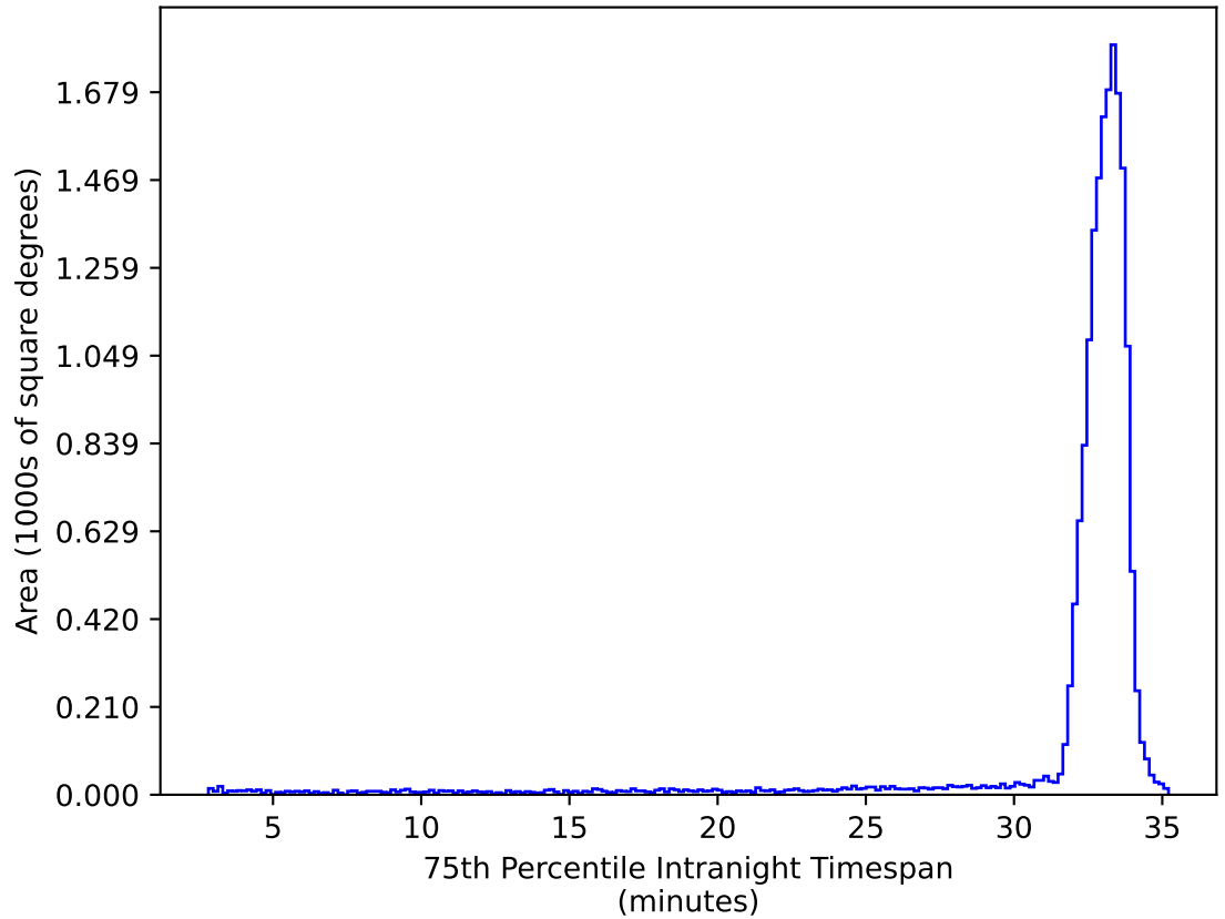
weather_cloudso30v3.4_10yrs WFD ug bands: 75th Percentile Intranight Timespan
