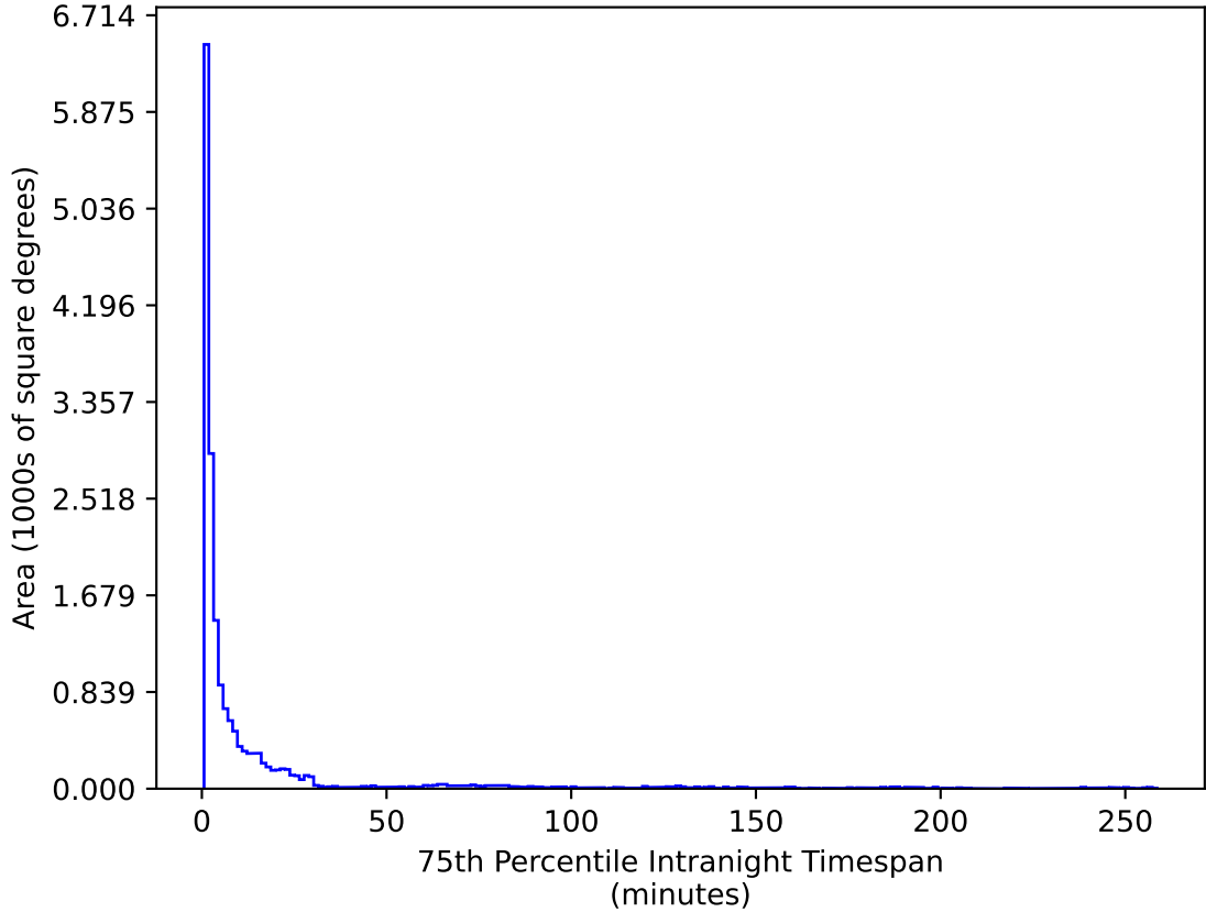
weather_cloudso30v3.4_10yrs WFD u band: 75th Percentile Intranight Timespan
