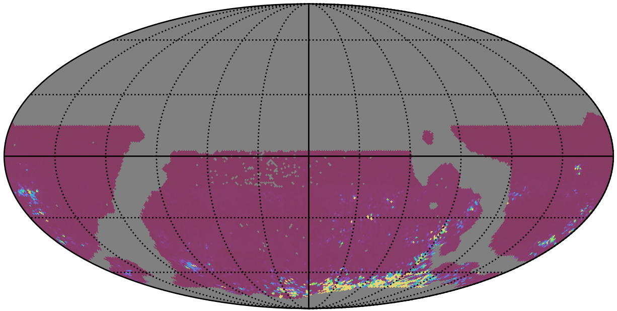
weather_cloudso30v3.4_10yrs WFD ri bands: 75th Percentile Intranight Timespan
