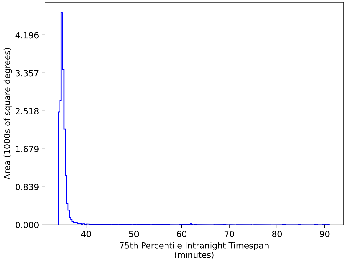
weather_cloudso30v3.4_10yrs WFD ri bands: 75th Percentile Intranight Timespan
