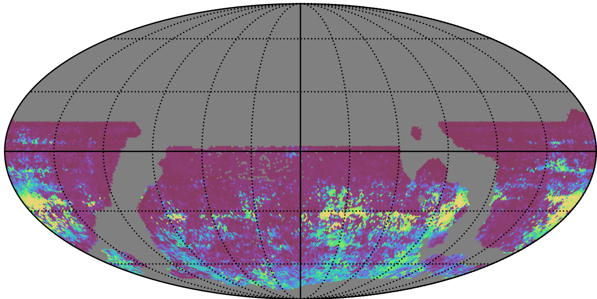
weather_cloudso30v3.4_10yrs WFD r band: 75th Percentile Intranight Timespan
