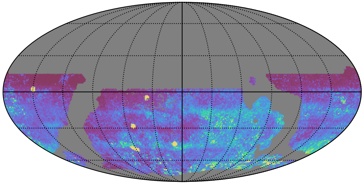
weather_cloudso30v3.4_10yrs WFD iz bands: 75th Percentile Intranight Timespan
