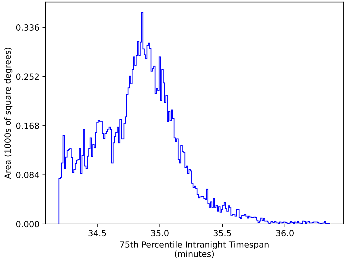
weather_cloudso30v3.4_10yrs WFD iz bands: 75th Percentile Intranight Timespan
