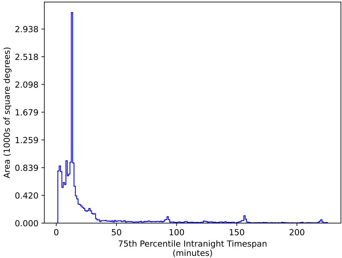
weather_cloudso30v3.4_10yrs WFD i band: 75th Percentile Intranight Timespan
