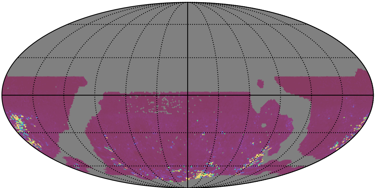
weather_cloudso30v3.4_10yrs WFD gr bands: 75th Percentile Intranight Timespan
