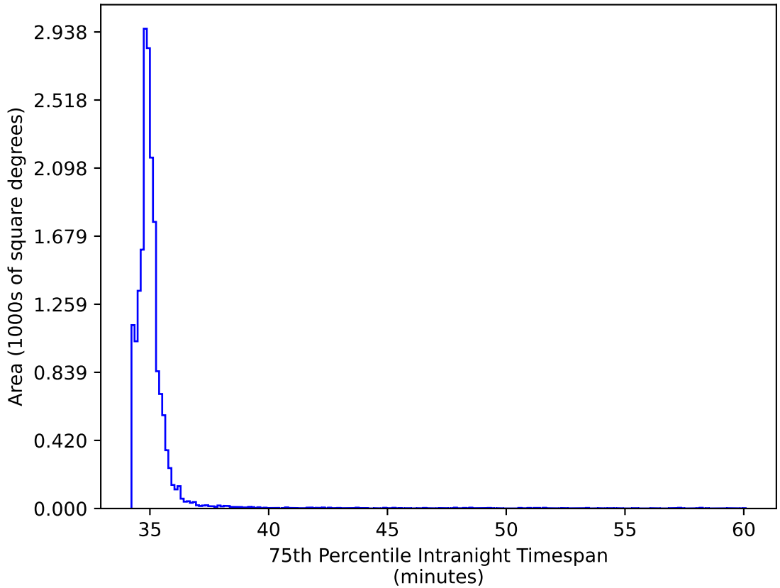
weather_cloudso30v3.4_10yrs WFD gr bands: 75th Percentile Intranight Timespan
