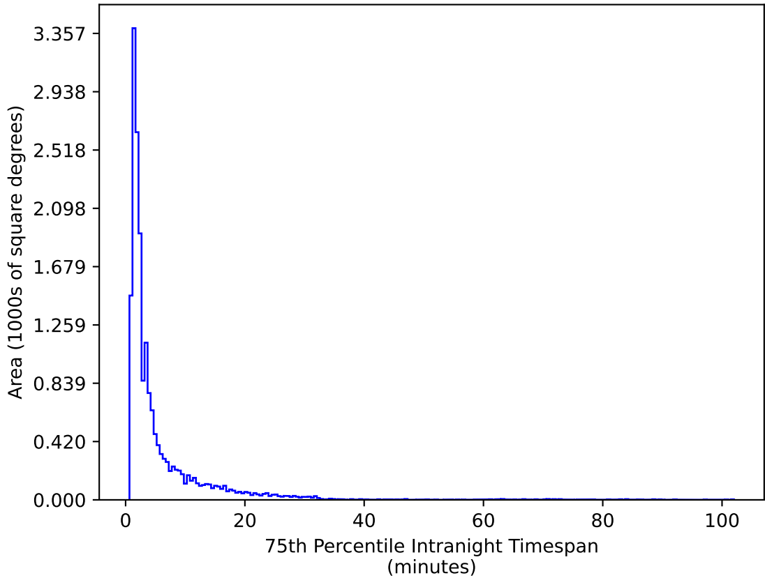
weather_cloudso30v3.4_10yrs WFD g band: 75th Percentile Intranight Timespan
